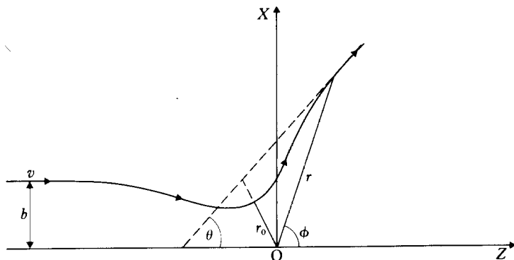
13.3 The classical path of a particle scattered by a centre of force situated at O.
